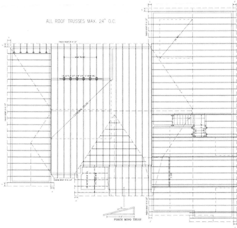
LOT 1 OLD VILLAGE ROOF FRAMING
