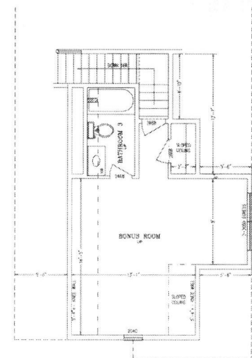
LOT 1 OLD VILLAGE 2ND FLR
